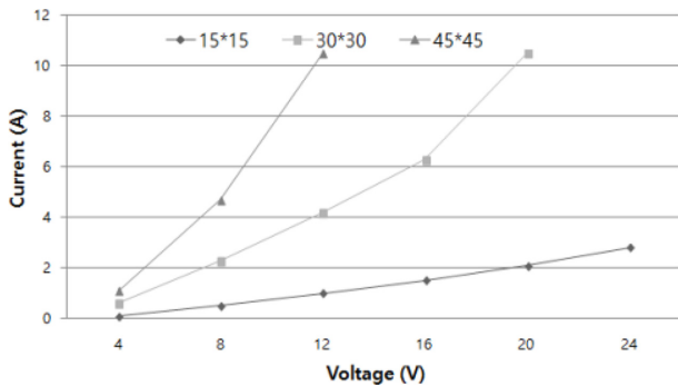
Fig. 4. The voltage and current according to the electrode size (EC 2.0, voltage: DC 0-24V, treated time: 30 sec).
